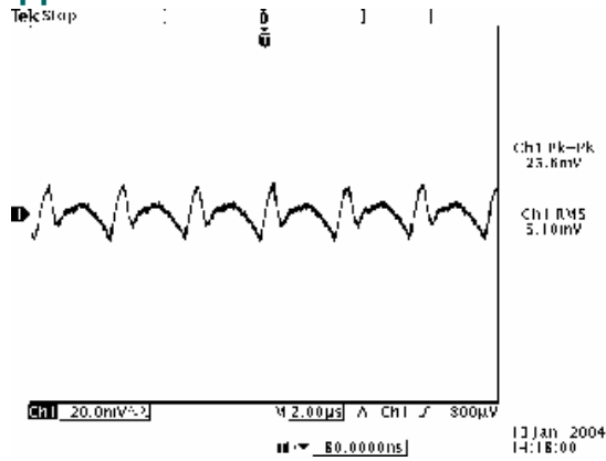
Ripple and noise at full load, V_{in}=5.0 V, V_o=0.7525 V
