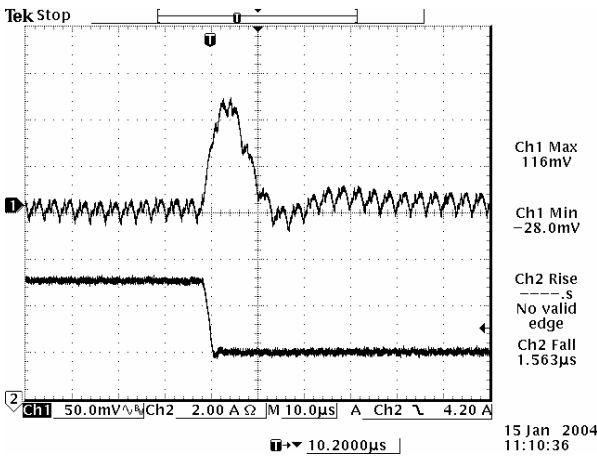
100% to 50% load step at V_{in}=5\text{ V} , V_o=1.5\text{ V}
