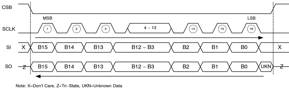
Figure 10. SPI Communications Frame Format
