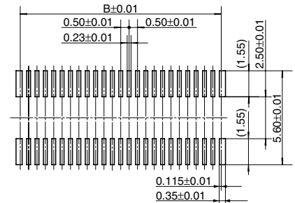
Recommended metal mask pattern Metal mask thickness: When 150 \mu m (Opening area ratio: 62%)
