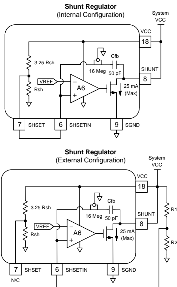
Figure 2. Shunt Regulator
