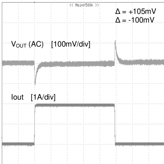
Figure 14. Transient Response (Vin=12V, Vout=3.3V, L=4.7μH, Cout=44μF, Iout=2A)
