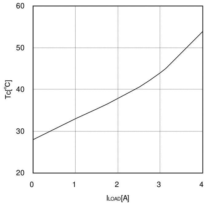
Figure 5. T C vs I LOAD (VIN=12V, Vout=3.3V, L=4.7μH, Cout=44μF)
