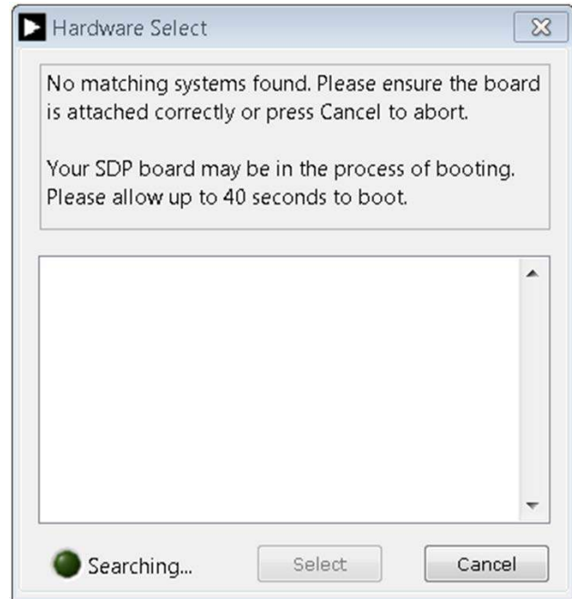
Figure 2. Connectivity Error
