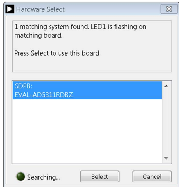
Figure 3. Hardware Select
