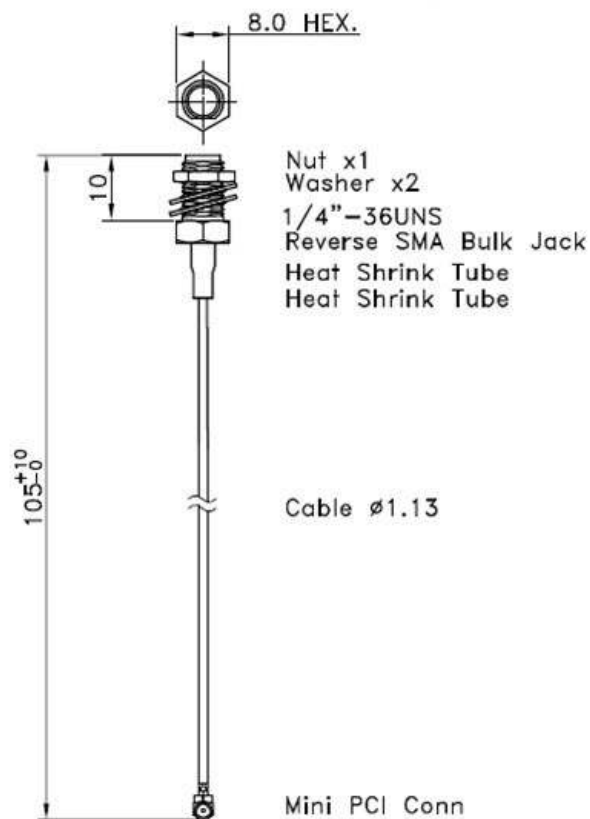
Figure 1 Physical Dimensions
