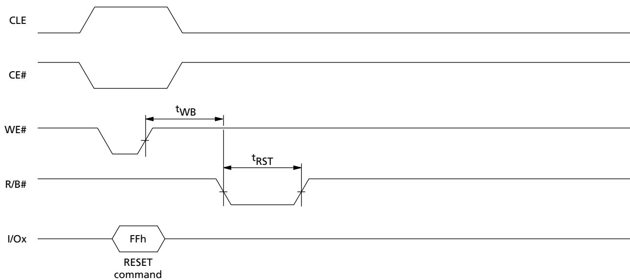
Figure 46: RESET Operation
