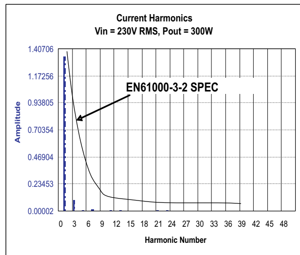
Figure 7. Current Harmonics
