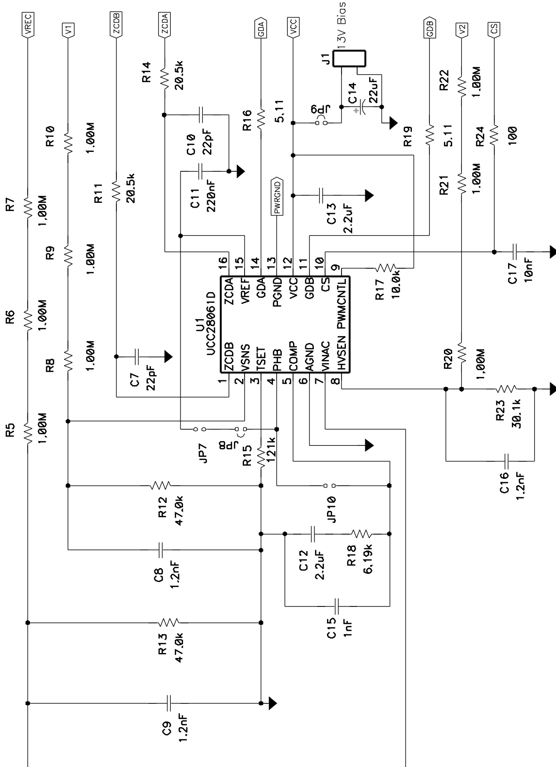
Figure 2. Controller Circuitry
