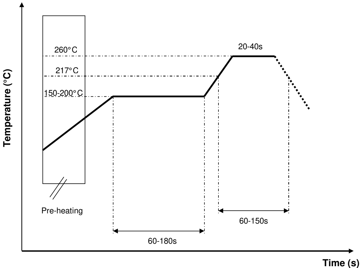
Typical Soldering Profile for Lead-free Process
