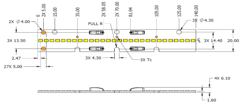
Figure 7: Drawing for EB Series Gen3 F90 140mm
