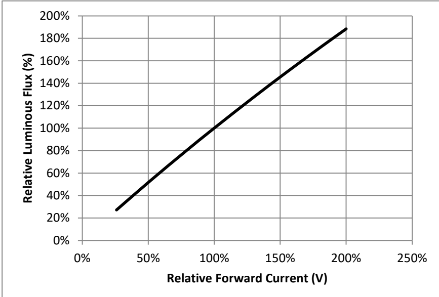
Figure 2: Relative Luminous Flux vs. Relative Forward Current, T_c=25^\circ\text{C}
