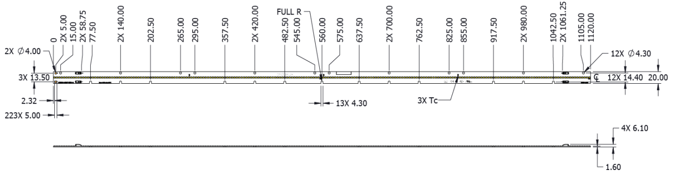
Figure 10: Drawing for EB Series F90 Gen3 1120mm
