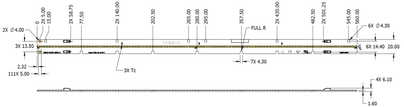
Figure 9: Drawing for EB Series Gen3 F90 560mm
