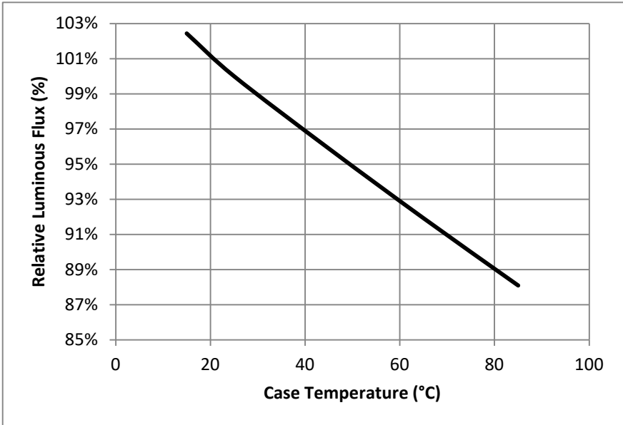
Figure 4: Relative Luminous Flux vs. Case Temperature
