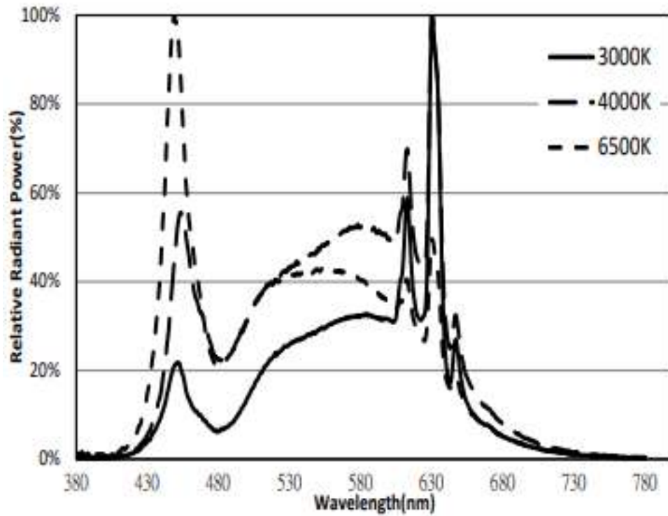
Figure 6: Typical Color Spectra, 90 CRI
