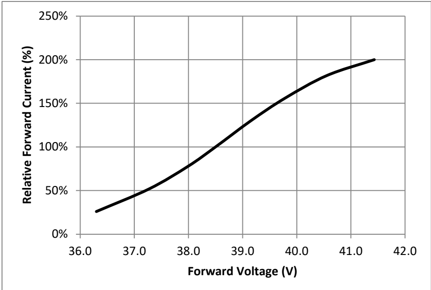
Figure 1: Relative Forward Current vs. Forward Voltage, T_c=25^\circ\text{C}
