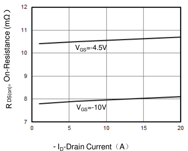
Figure 4. R_{DS(on)} Drain Current
