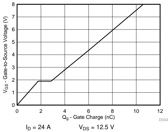
Figure 4. Gate Charge
