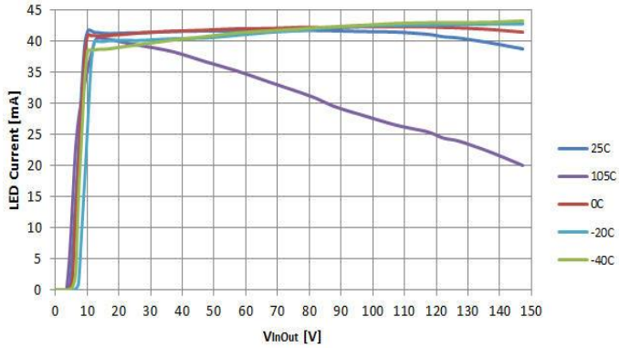
Figure 10. LED Current (-40°C to +105°C) vs. V_{IN\_OUT}
