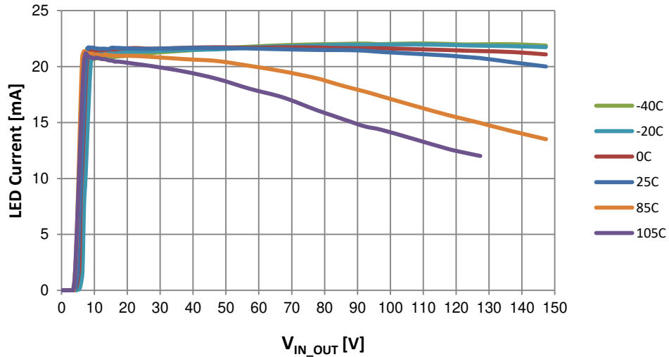
Figure 1. LED Current (-40°C to 105°C) vs. V IN_OUT
