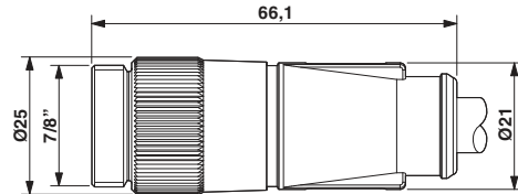
Dimensioned drawing
