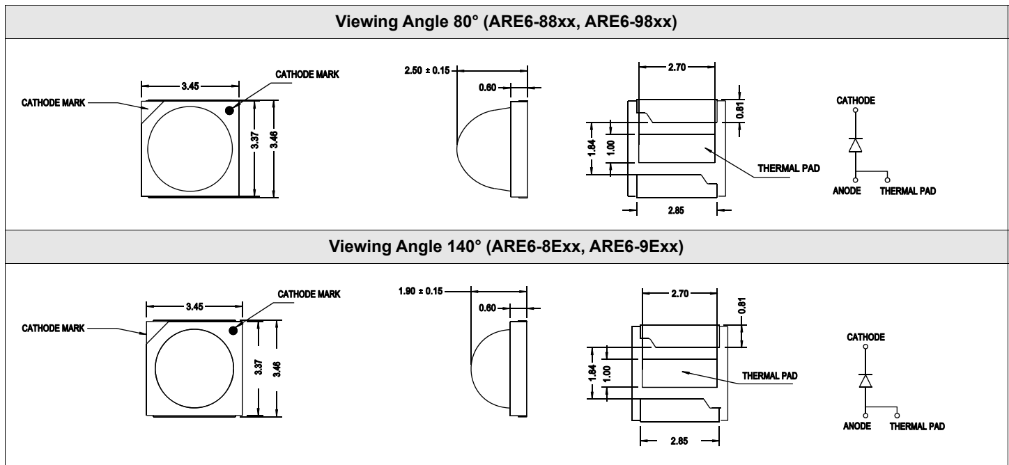
Figure 1: Package Drawing
