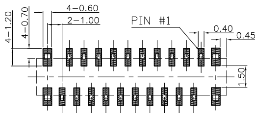
P.C.B LAYOUT A TYPE (REFERENCE) TOL:±0.05
