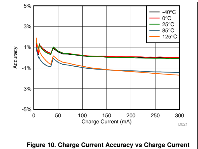
Figure 10. Charge Current Accuracy vs Charge Current
