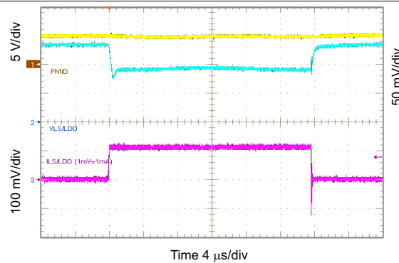
Figure 92. 3.3 V_{LSLDO} Load Transient, 0 to 100 mA
