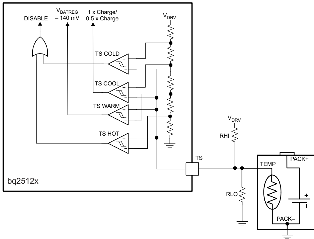
Figure 18. TS Circuit
