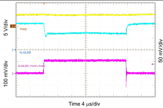
Figure 91. 2.5 V_{LSLDO} Load Transient, 0 to 100 mA
