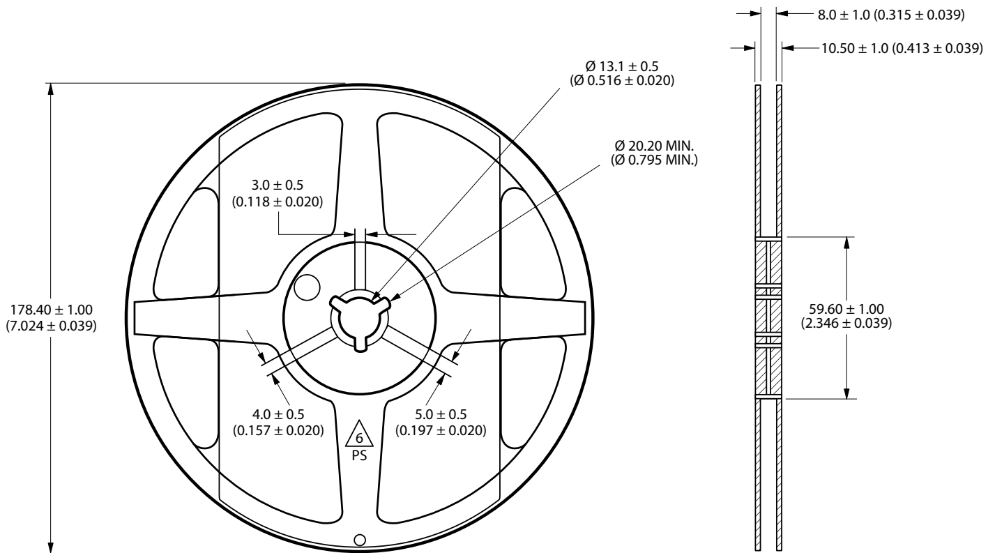
Figure 10: Reel Dimensions
