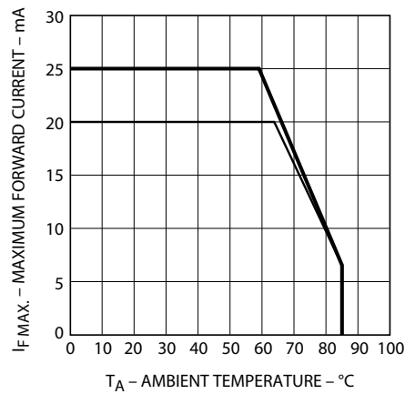
Figure 4: Maximum Forward Current versus Ambient Temperature
