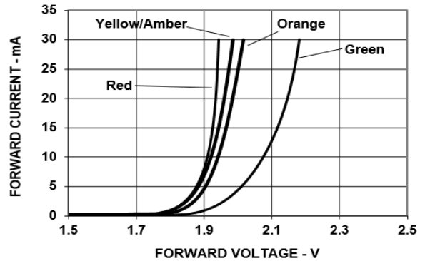
Figure 2: Forward Current versus Forward Voltage
