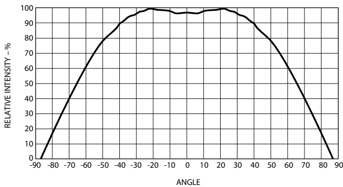
Figure 5: Relative Intensity versus Angle
