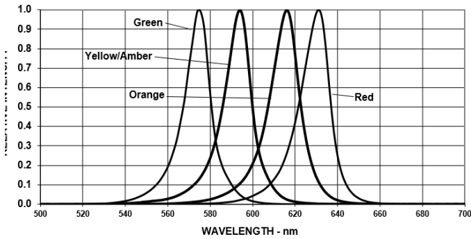
Figure 1: Relative Intensity versus Wavelength
