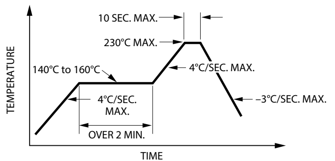
Figure 6: Recommended Reflow Soldering Profile
