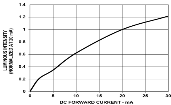
Figure 3: Luminous Intensity versus Forward Current
