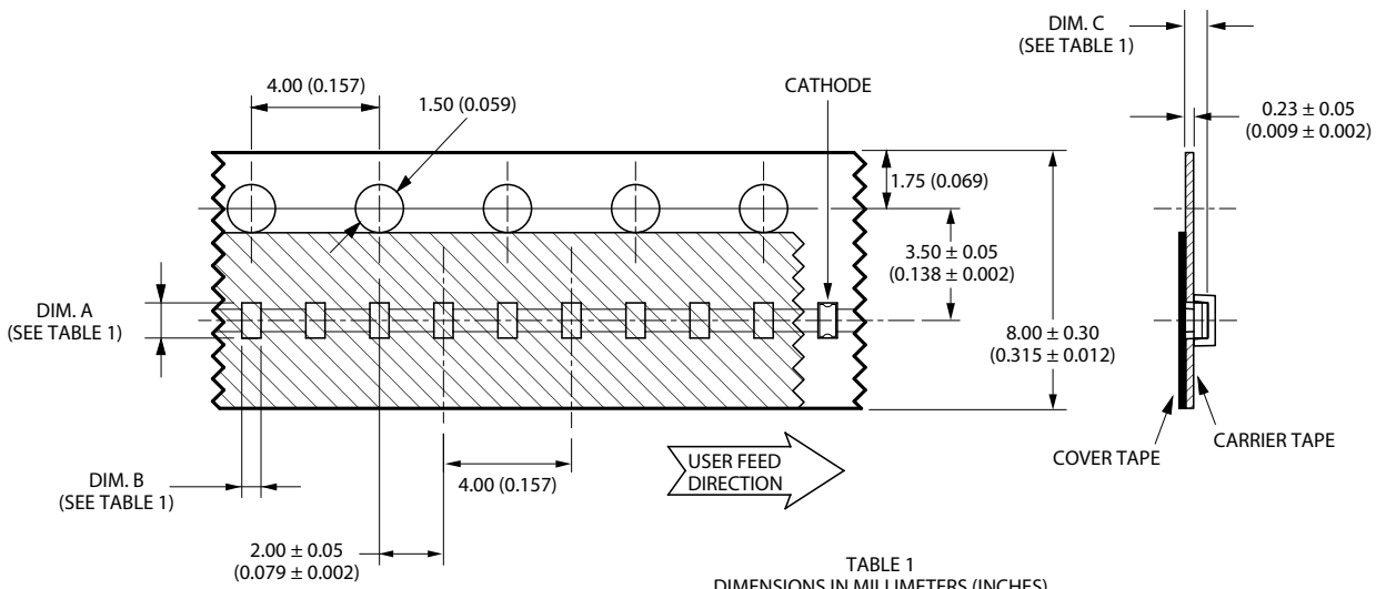
Figure 11: Tape Dimensions
