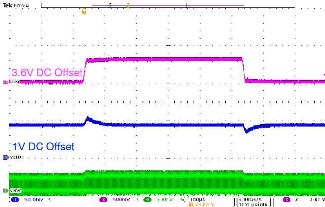
Figure 13. Line Transient, 3.6 V↔4.2 V, 1A, 10 µs Edge
