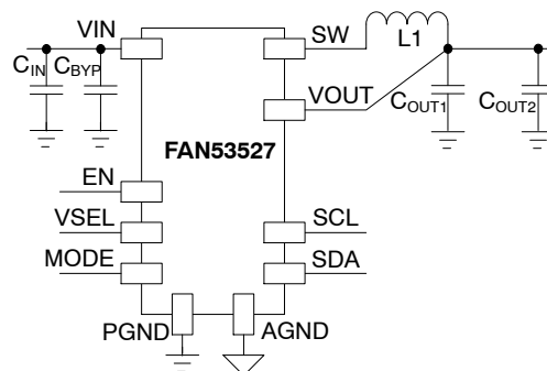
Figure 1. Typical Application
