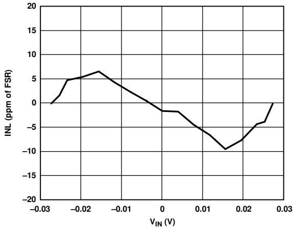
Figure 14. INL (Gain = 128)
