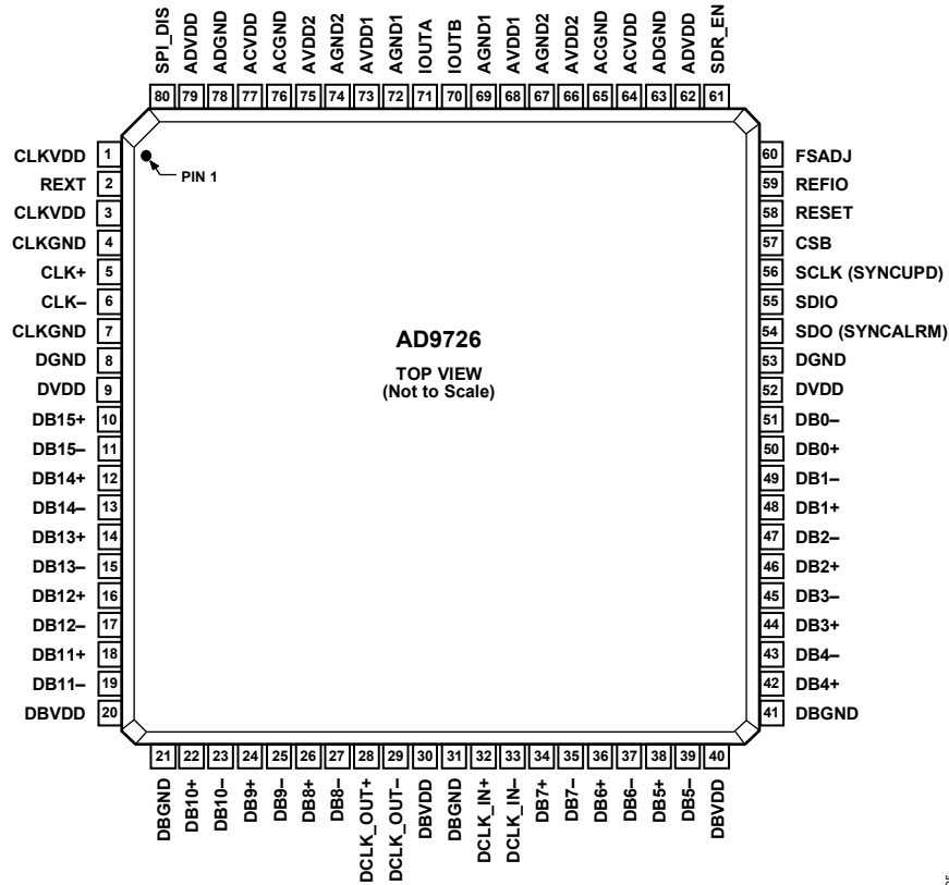
Figure 7. Pin Configuration
