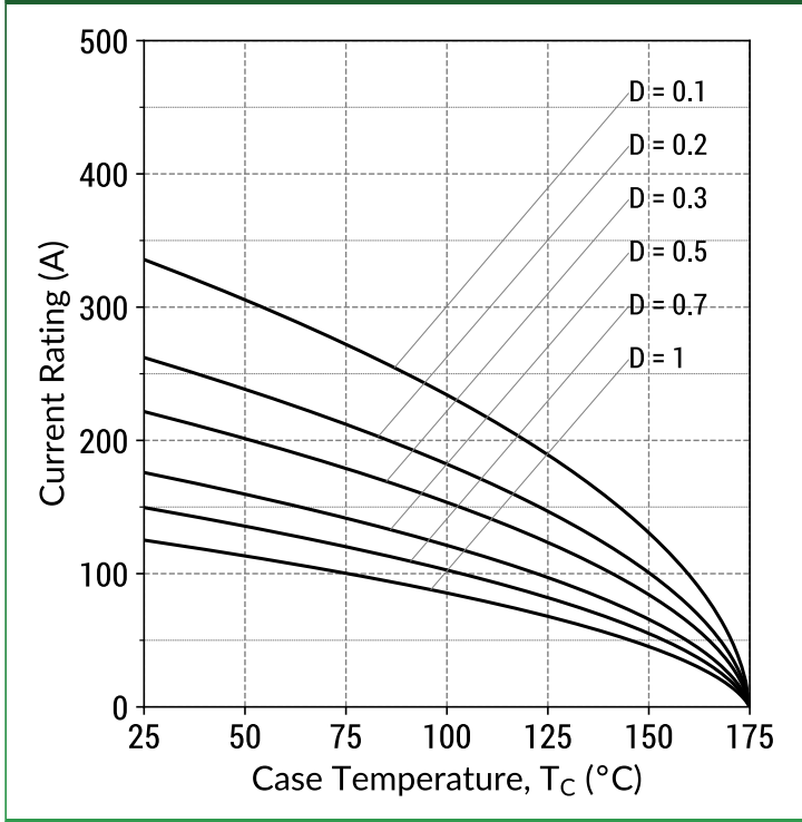
Figure 5: Current Derating Curves (Maximum V_F )
