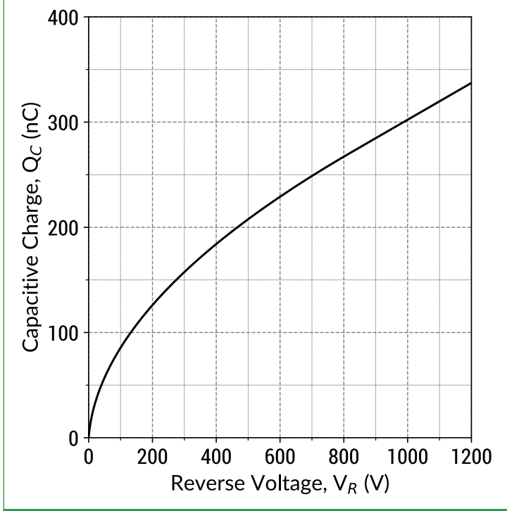
Figure 7: Typical Capacitive Charge vs Reverse Voltage Characteristics
