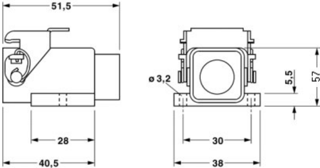
Dimensioned drawing
