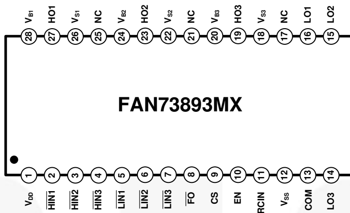
Figure 3. Pin Assignments
