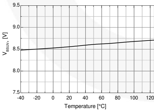
Figure 20. V_{BS} UVLO+ vs. Temperature
