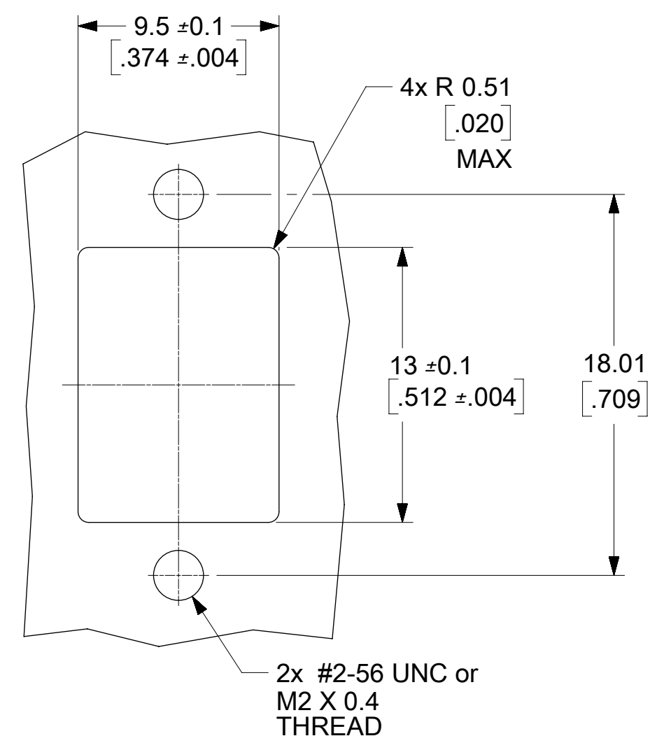
RECOMMENDED MOUNTING PATTERN
