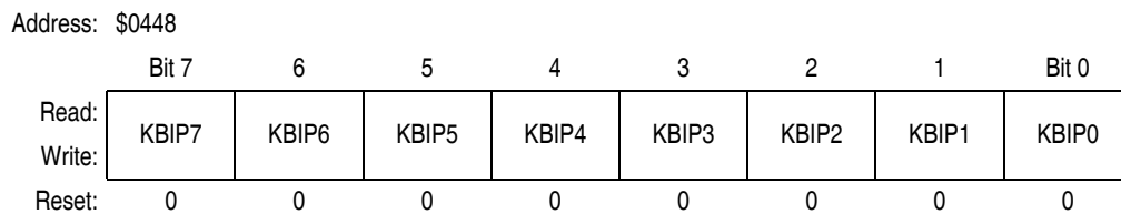
Figure 9-6. Keyboard Interrupt Polarity Register (INTKBIPR)
