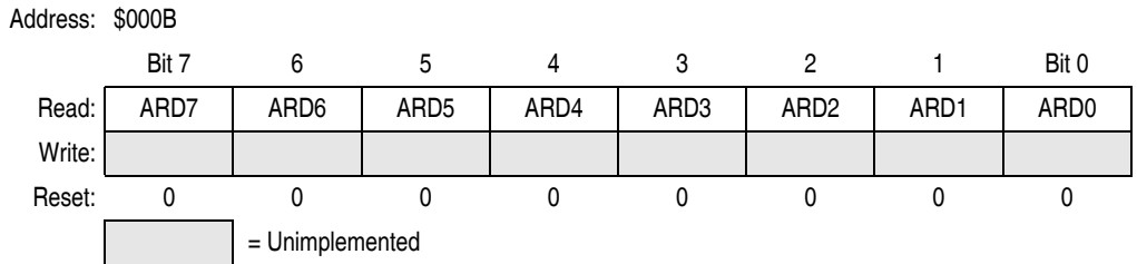
Figure 13-20. ESCI Arbiter Data Register (SCIADAT)
