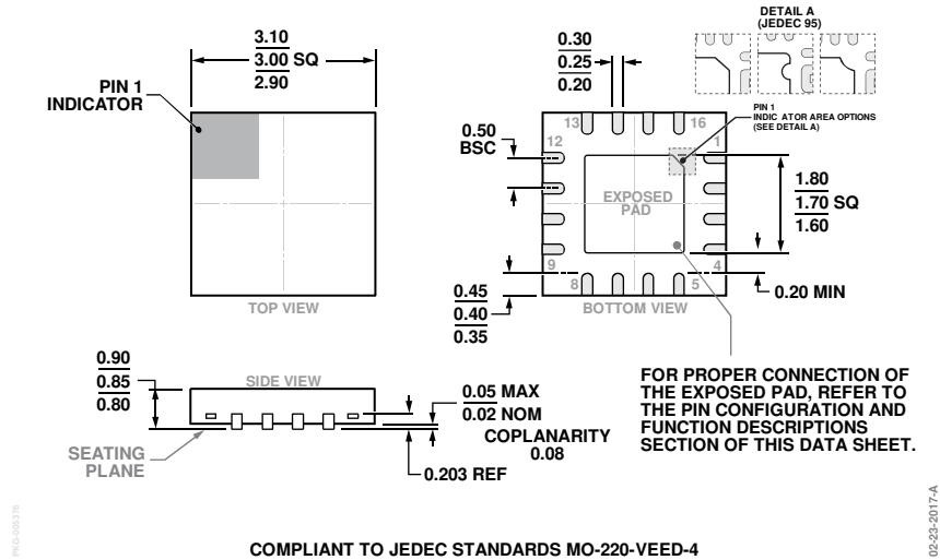
Figure 10. 16-Lead Lead Frame Chip Scale Package [LFCSP] 3 mm × 3 mm Body and 0.85 mm Package Height (CP-16-51) Dimensions shown in millimeters
