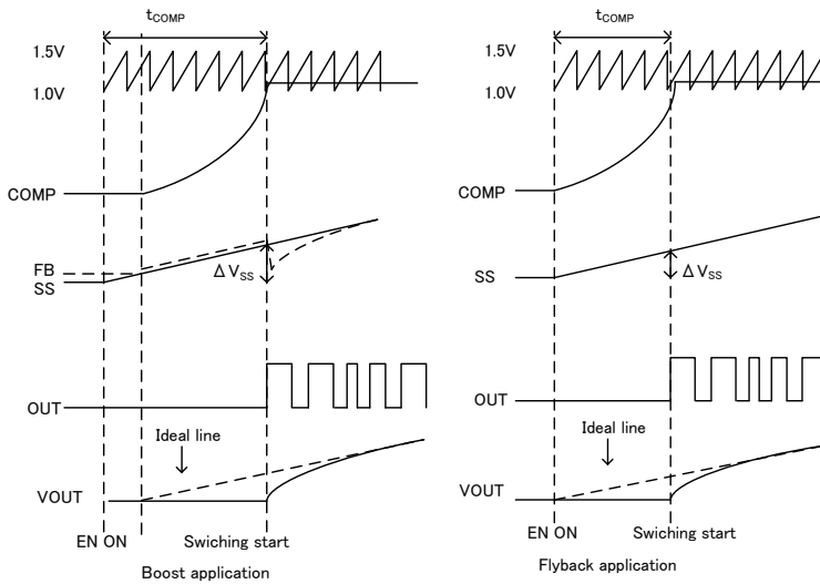
Figure 9. Output voltage starting diagram
