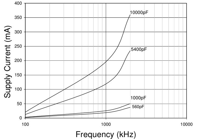
Fig. 23 Supply Current vs. Frequency V_{\text{SUPPLY}} = 20\text{V}
