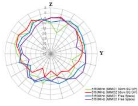
YZ Plane
