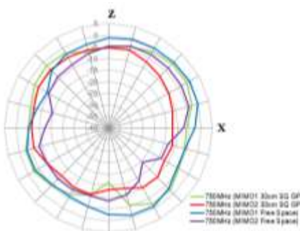
XZ Plane
