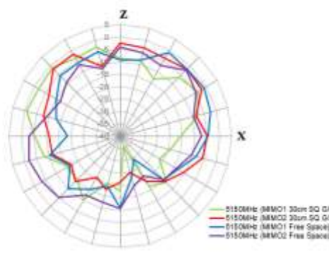
XZ Plane
