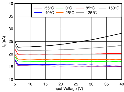
Figure 6-25. Quiescent Current ( I_Q ) vs V_{IN}
