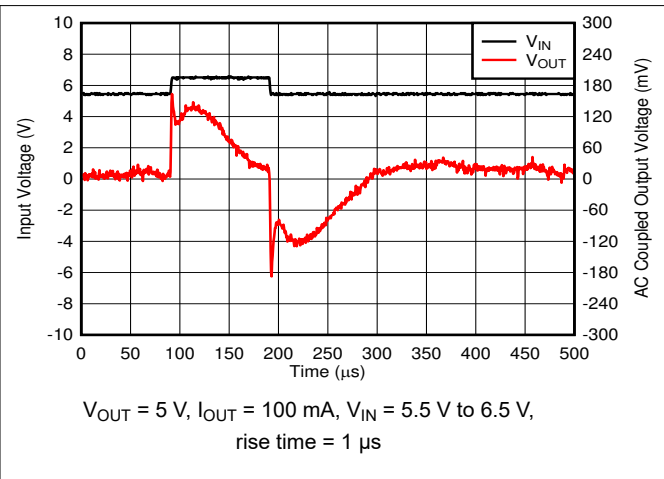
Figure 6-14. Line Transients
