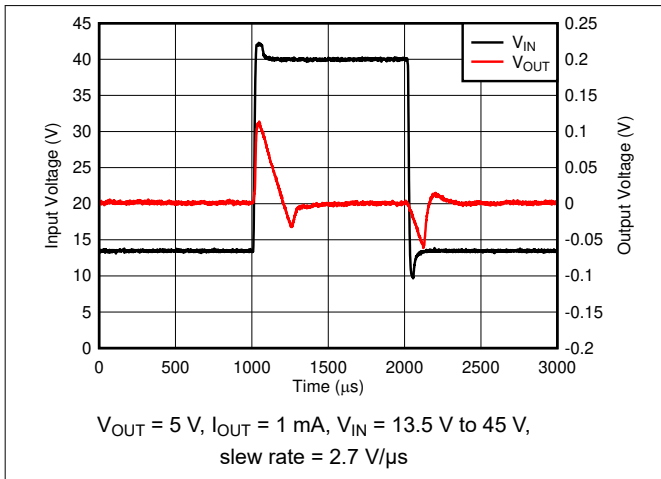
Figure 6-13. Line Transients
