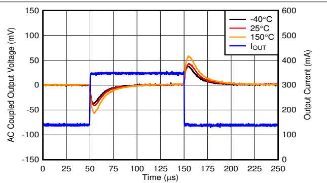
Figure 8-10. Transient Response
