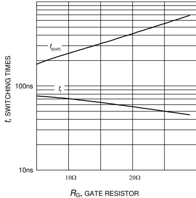
Figure 10. Typical switching times as a function of gate resistor (inductive load, T_J = 175^\circ\text{C} , V_{CE}= 400\text{V} , V_{GE} = 0/15\text{V} , I_C = 40\text{A} , Dynamic test circuit in Figure E)
