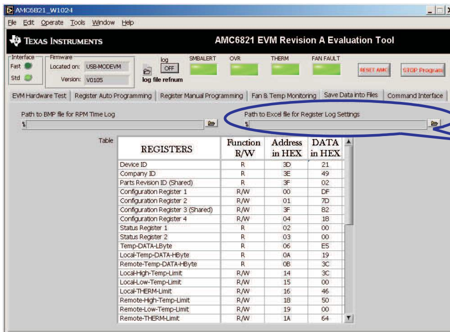
Figure 19. Register Settings
