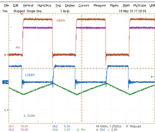
CH1: HIDRV, 10 V/div; CH2: LODRV, 5 V/div; CH3: PHASE, 10 V/div; CH4: inductor current, 2 A/div, 400 ns/div Figure 6. Continuous Conduction Mode Switching Waveforms
