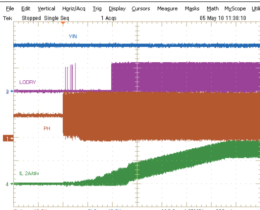
CH1: PHASE, 10 V/div; CH2: Vin, 10 V/div; CH3: LODRV, 5 V/div; CH4: inductor current, 2 A/div, 2 ms/div Figure 4. Current Soft-Start
