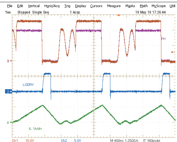
CH1: HIDRV, 10 V/div; CH2: LODRV, 5 V/div; CH3: PHASE, 10 V/div; CH4: inductor current, 1 A/div, 400 ns/div Figure 7. Cycle-by-Cycle Synchronous to Nonsynchronous
