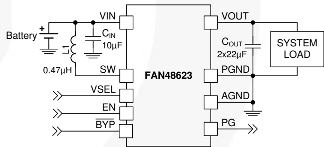
Figure 1. Typical Application
