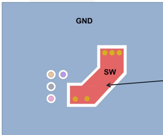
Figure 44. Layer 3
