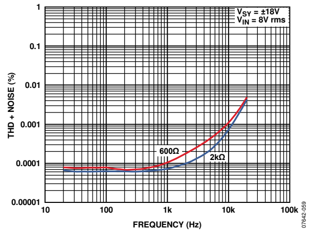
Figure 61. THD + Noise vs. Frequency
