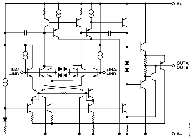
Figure 70. Simplified Schematic
