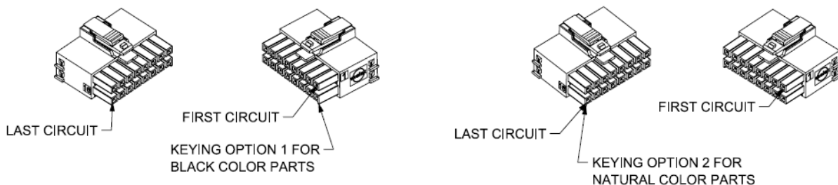
KEYING OPTION 1
