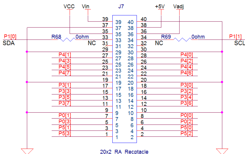
Figure 3-12. CY3280-CPM1 Board Connector
