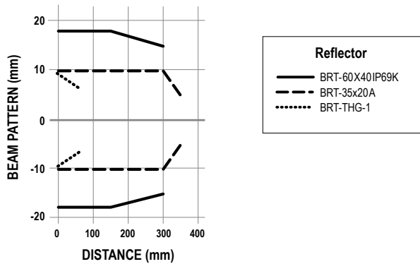
Figure 4. Beam Pattern
