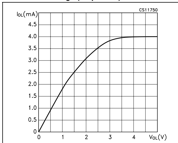
Figure 10. Receiver output current vs. output voltage (output low)
