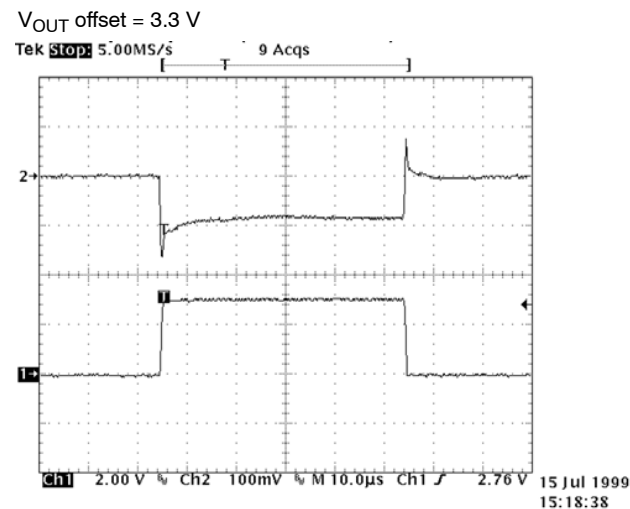
Figure 10. Load Step Response
