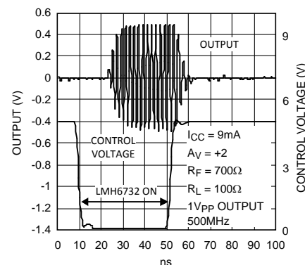
Figure 2. Turn-On/Off Characteristics
