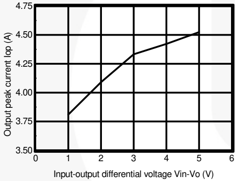
Figure 29. Output Peak Current vs. Input-Output Differential Voltage
