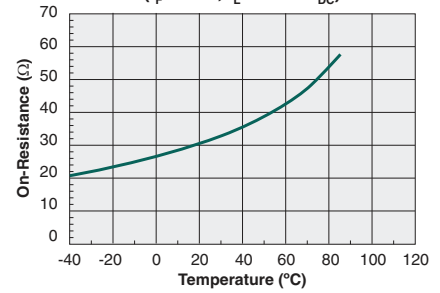
Typical On-Resistance vs. Temperature ( I_F=2mA, I_L=100mA_{DC} )
