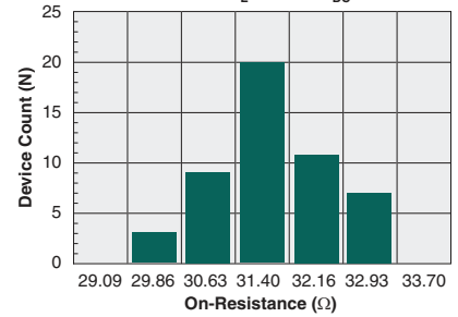
Typical On-Resistance Distribution (N=50, I_L=100\text{mA}_{DC} )
