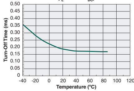
Typical Turn-Off Time vs. Temperature ( I_L=100mA_{DC} )
