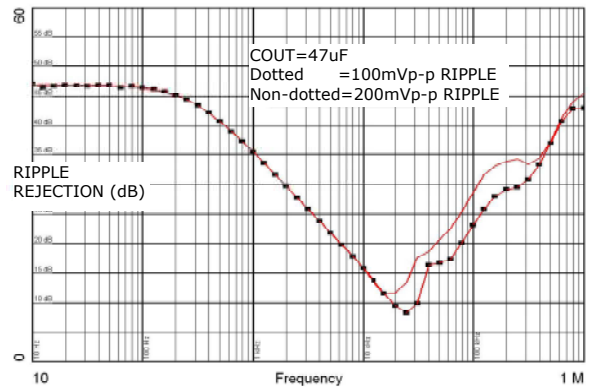
Fig. 13: PSRR, 50mA, 1.5VIN, 1VOUT, 47uF COU
