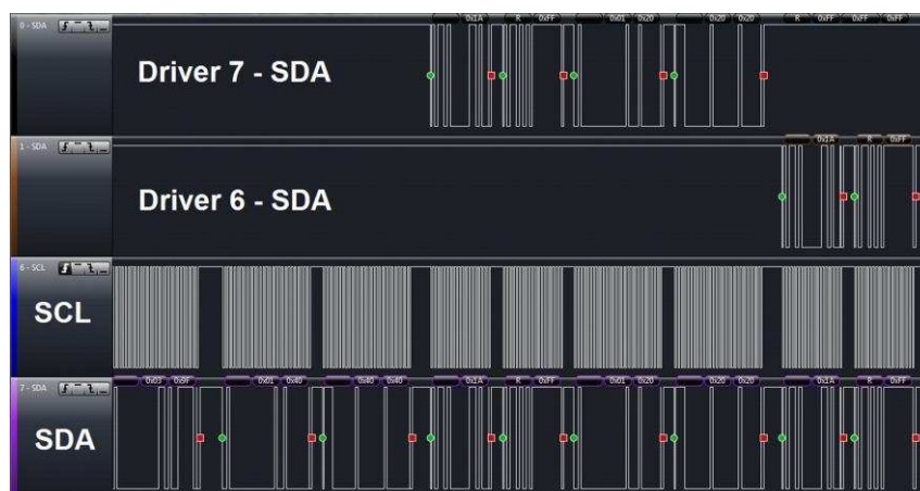
Figure 10. TCA9548A Logic Analyzer Operation
