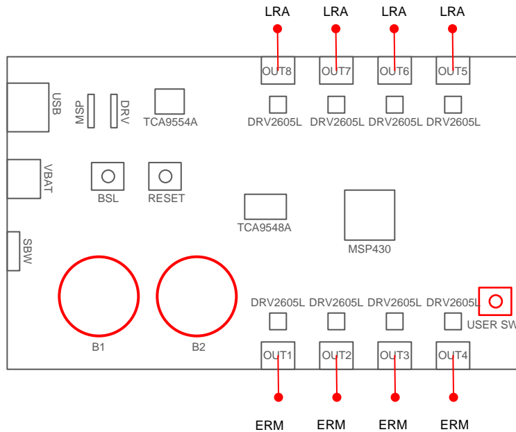
Figure 4. Board With Actuator Setup
