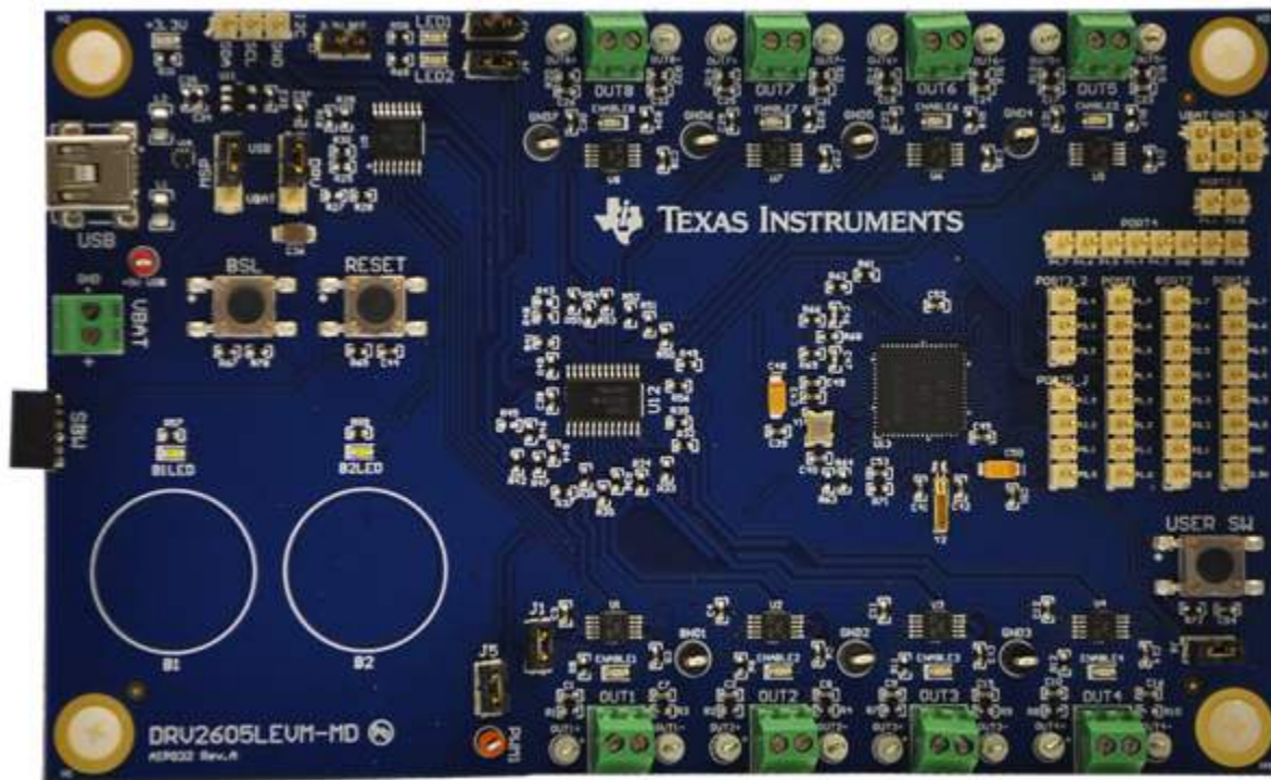
Figure 1. DRV2605LEVM-MD
