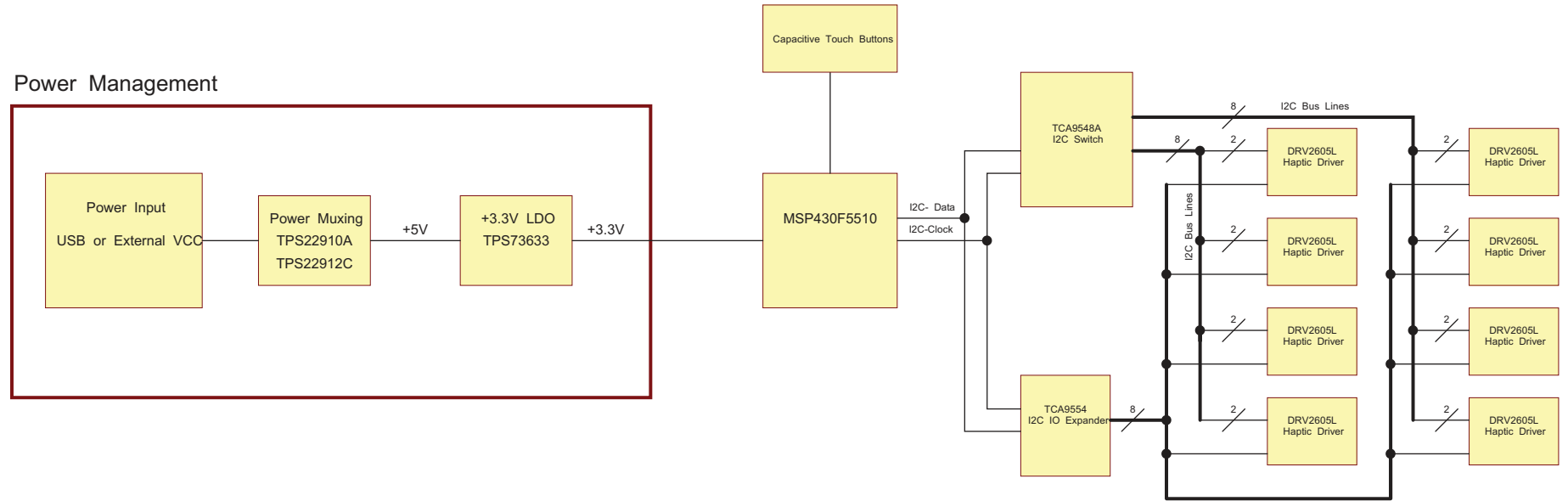
Figure 20. Schematic Block Diagram
