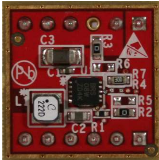
Figure 1. SMP-TPS61201-MVK Submodule
