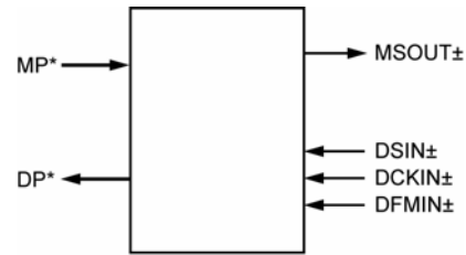
Figure 5. Loopback Function
