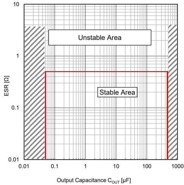
Figure 51. Output Capacitance C_{OUT} , ESR Available Area (-40 °C ≤ T j ≤ +150 °C, 4.5 V ≤ V IN ≤ 42 V, V EN = 5 V, I OUT = 0 mA to 150 mA)
